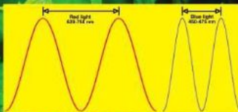
Figure 1: As distance between peaks changes, so does light's visible color.
